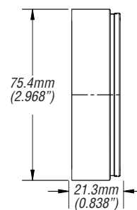
Achromatic Diopter 5.6oz (159g) (72mm Filter Thread)
