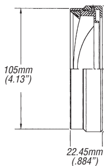
.6X Wide Angle Adapter 7oz (200g) (102mm Filter Thread)
