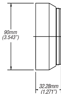
.8X Wide Angle Converter 10oz (283.5g) (86mm Filter Thread)
